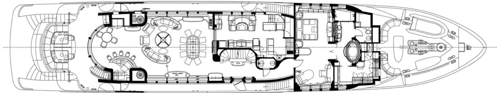
MAIN DECK
